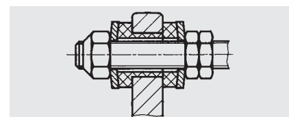
Sound damping outer and inner restraint (lateral expansion joint)
