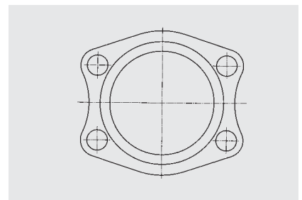
Flange as per SAE standard (type GR-SAE)
