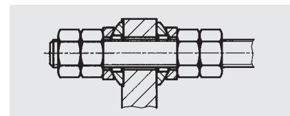
Outer and inner restraint with spherical washer and conical seat (lateral expansion joint)
