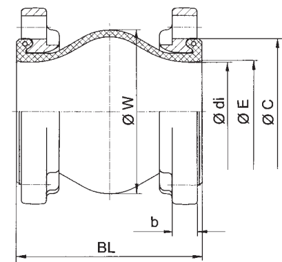
Type GR-SAE Universal expansion joint
