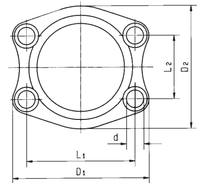
Flange according to SAE-standard
