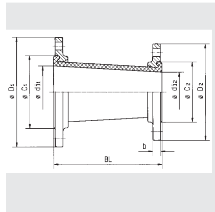
Type G Conical lateral expansion joint with rotating flanges
