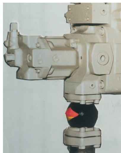
STENFLEX® type GR-SAE in a low-pressure hydraulic system
